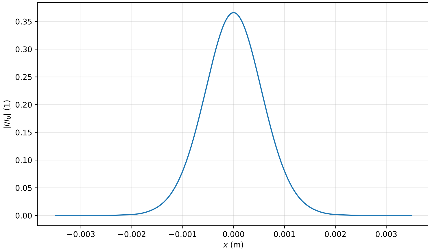
Intensity profile I(x, y = 0, z = 3.344m)/I_0 , P_{in}=0.3P_{cr} , artificial time
